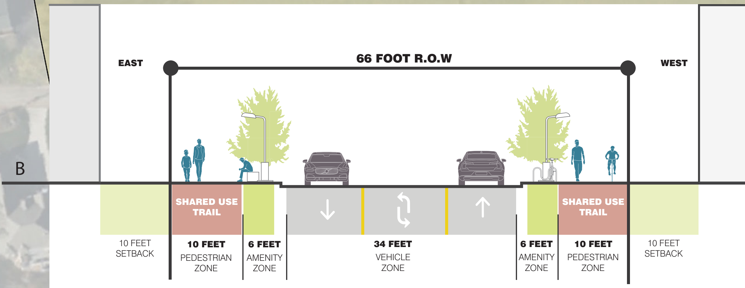
TYPICAL BACON TO OSTERHOUT CROSS-SECTION
