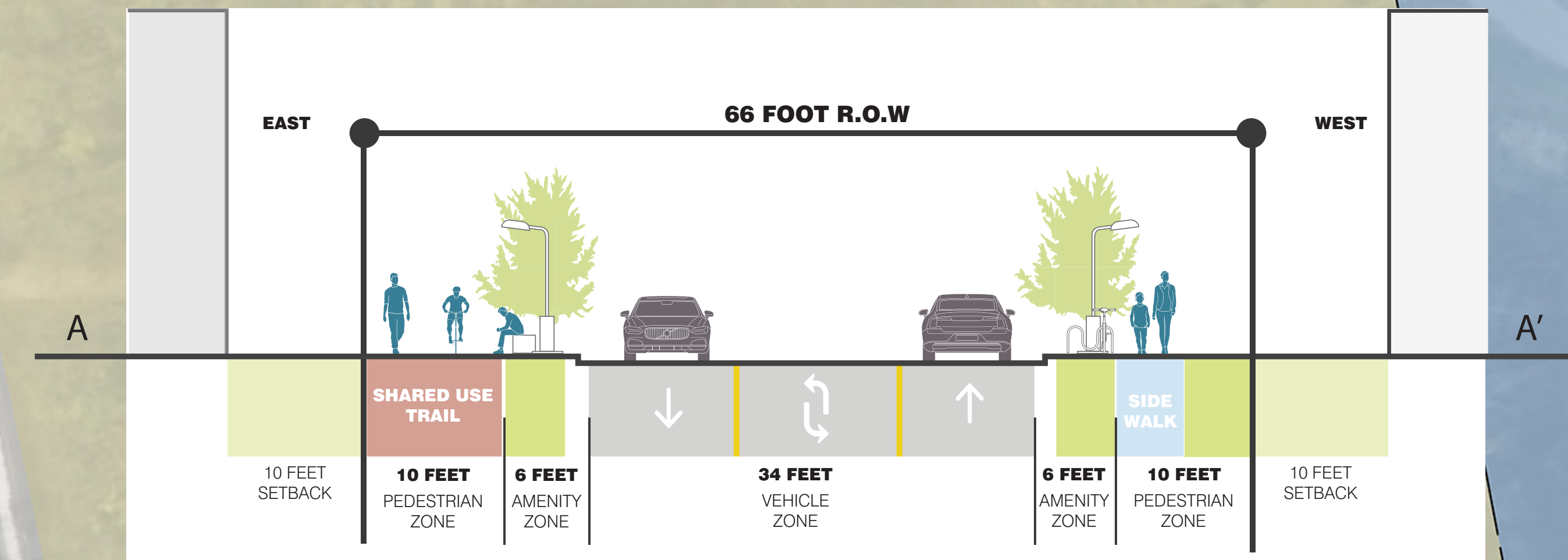
TYPICAL LAKEVIEW TO BACON CROSS-SECTION
