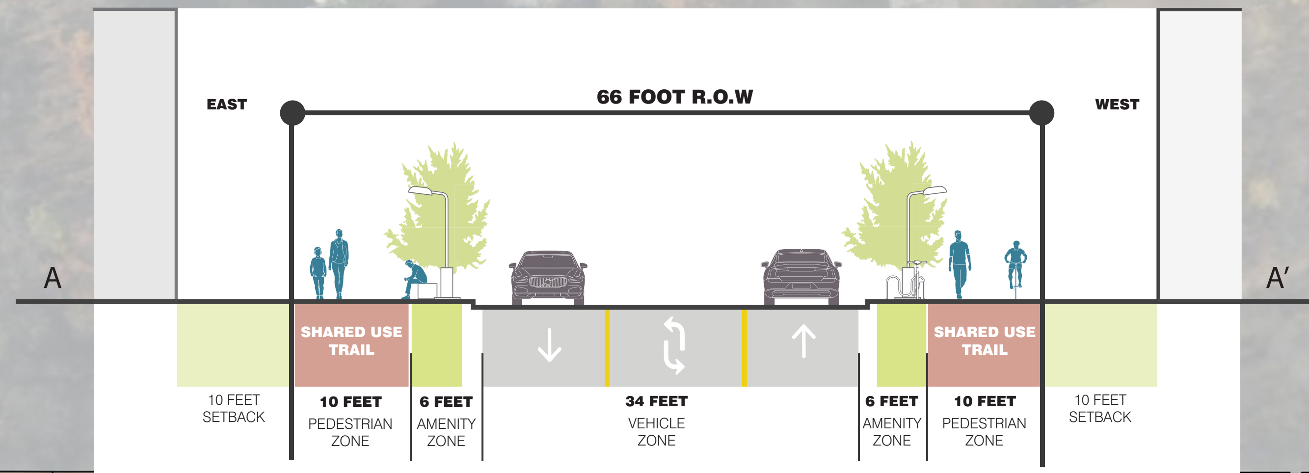
TYPICAL NORTH CROSS-SECTION
